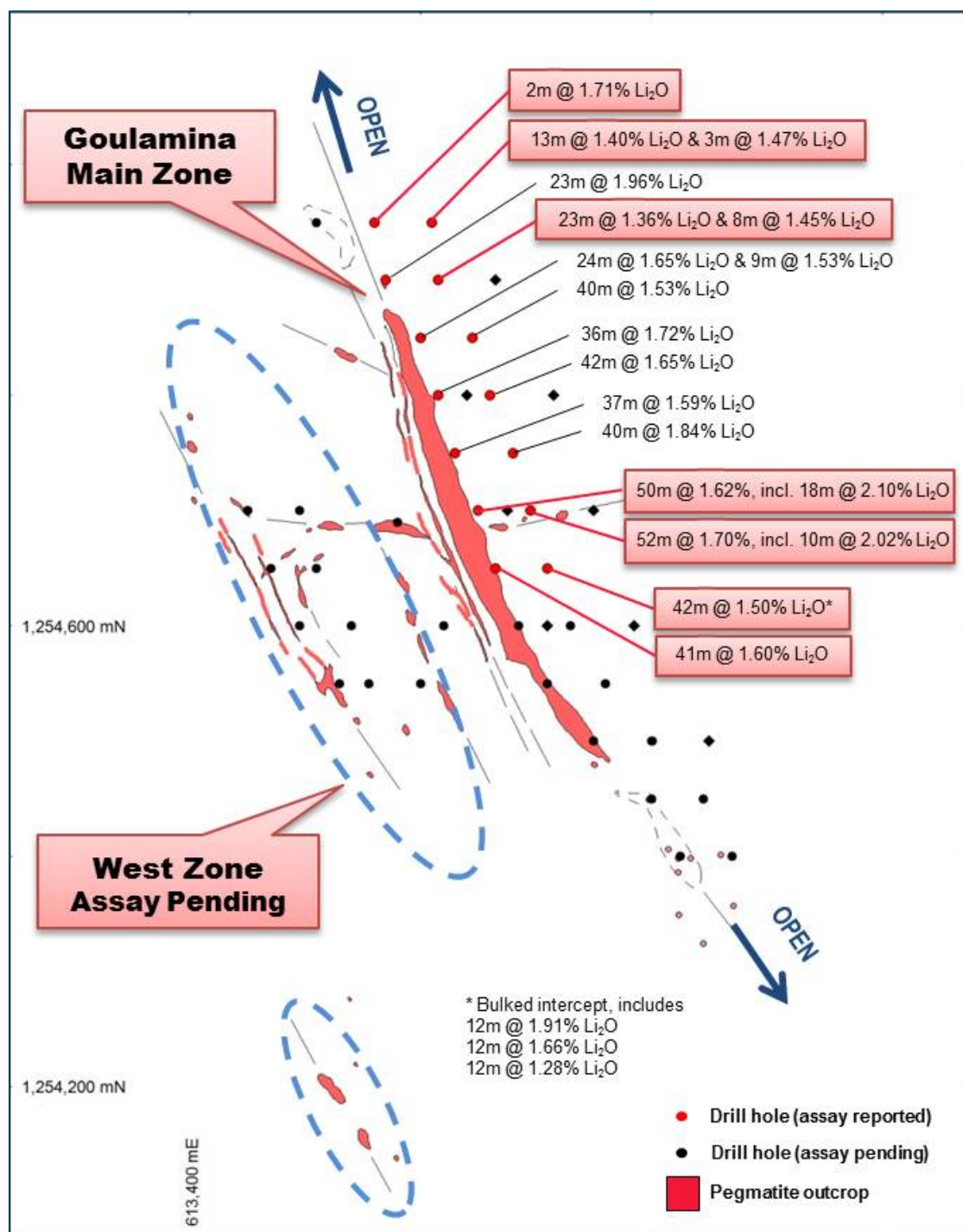
Figure 1. Goulamina Deposit. Lithium pegmatite outcrop map with drill hole locations and reported drill intersections (red).
